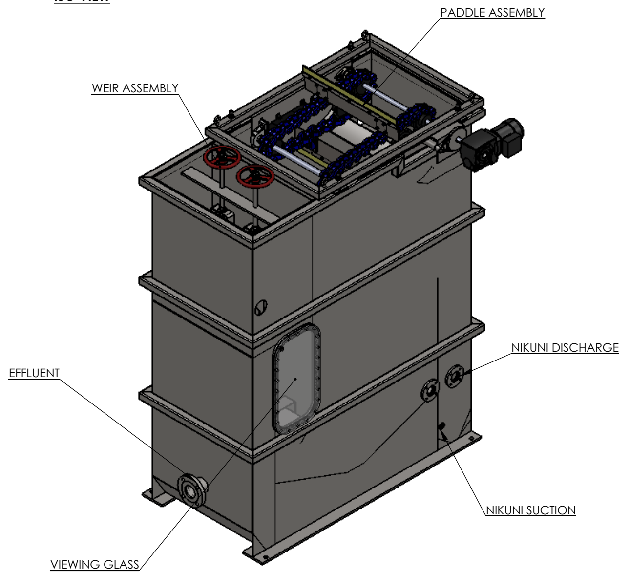
ISO VIEW
